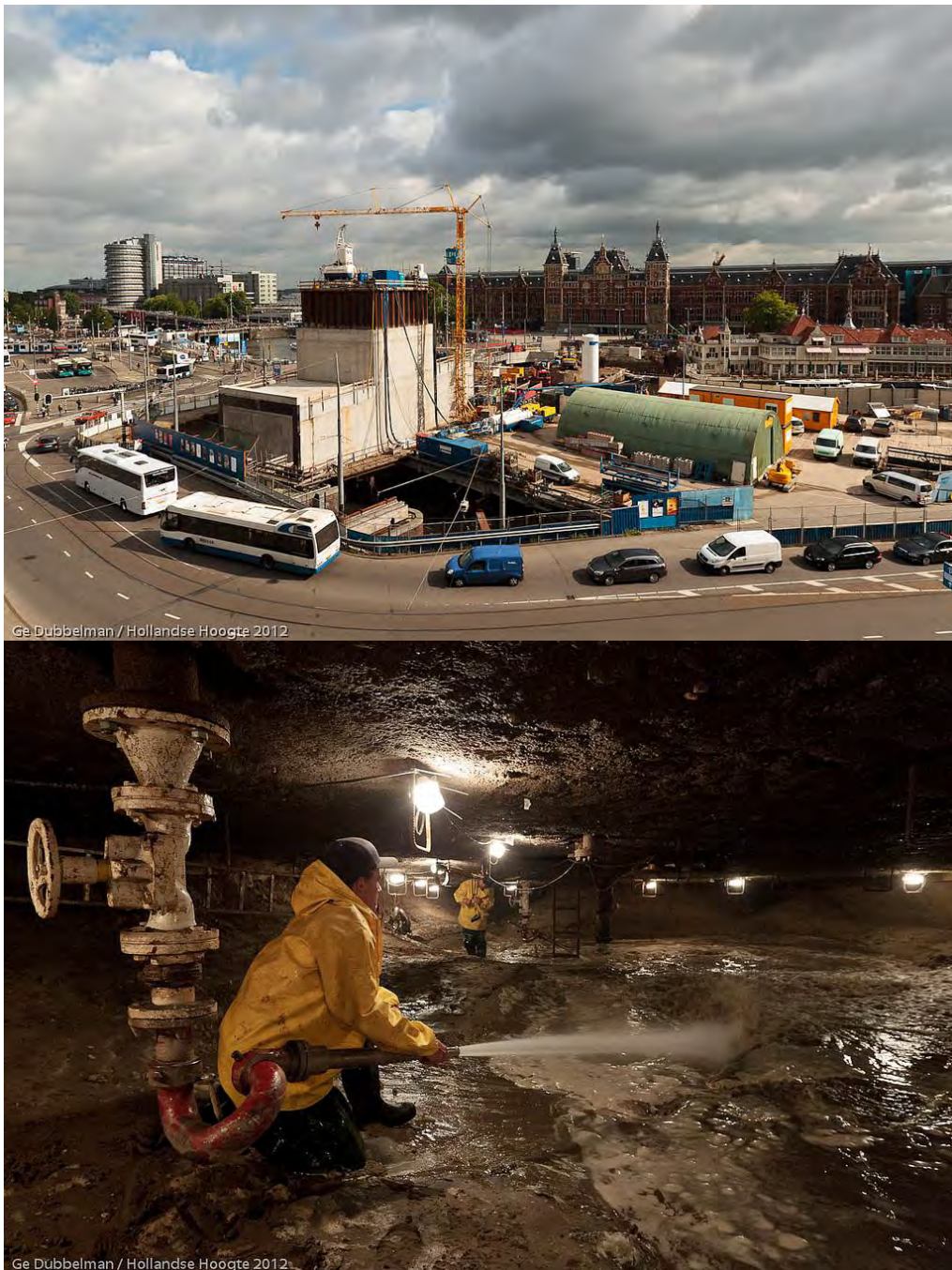
Figure Caisson at surface level (top) and excavation below caisson (bottom)
