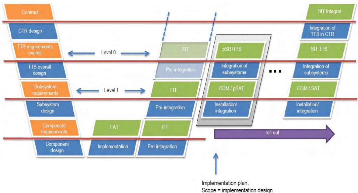
Figure V-model design traffic and tunnel systems 2nd Coentunnel.
