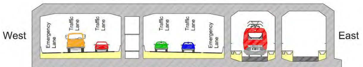
Figure cross section of the Fehmarnbelt tunnel.
