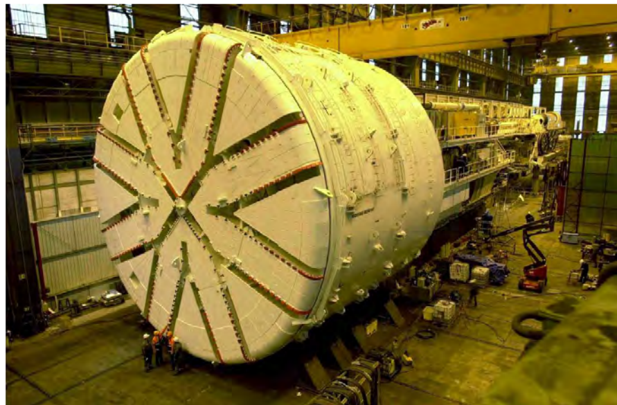
Figure: The 14.5m diameter TBM for the Groene Hart tunnel
