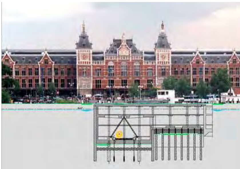
Figure: Schematic cross-section of the metro lines and entrance hall South Side
