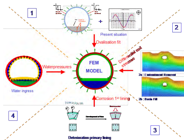
Figure: Calculation strategy Metro Lisbon
