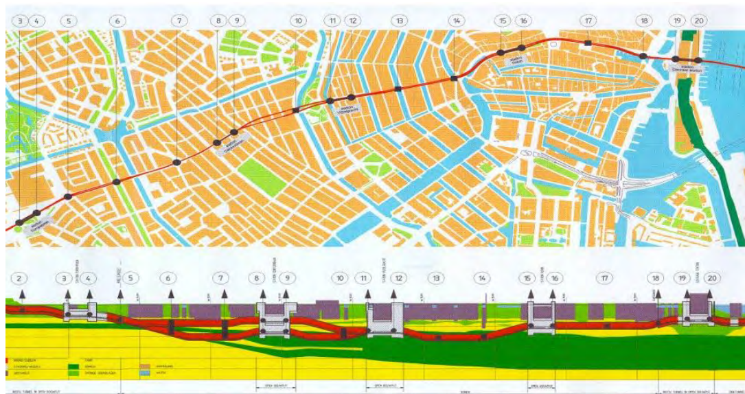
Figure: Plan and alignment of bored tunnel section
