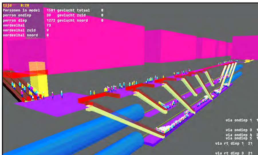
Figure general safety concept for tunnels and all underground stations, including many evacuation and transfer modelling and CFD simulations.
