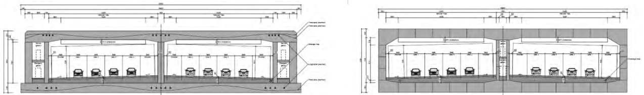
Figure; examples of options (structurally and geometrically) that were studied
